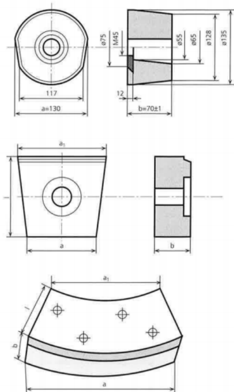
Grinding segment with thread
