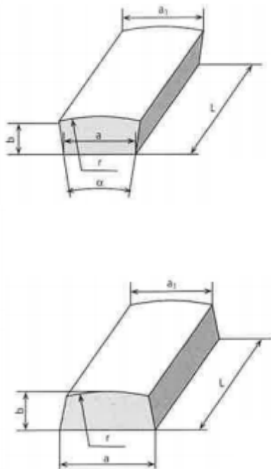
Grinding segment without thread
